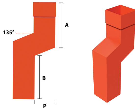
MAXIMUM PROJECTION OF SWAN NECKS
