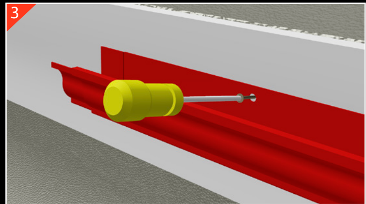
Once the position is established the first length can be fixed level, directly through the back of the gutter by 38 x 5 stainless steel screws (Guttercrest GM1).
