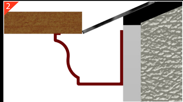
Alternatively use a spirit level against the lowest point of the roof tile to determine the position the gutter is fixed.*
