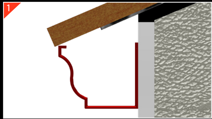
A straight edge can be placed along the pitch of the roof to determine the position (height) of the gutter.
