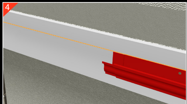
Next use a string / laser line, to determine the position of the remaining gutter lengths in the run. We recommend a level fall, if a fall is required - max. 1 : 600.
