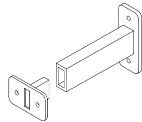
Mullion bracket
