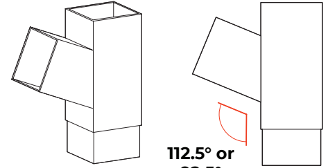
112.5° branch shown
