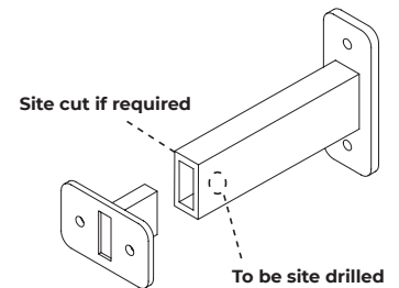
Mullion Bracket
