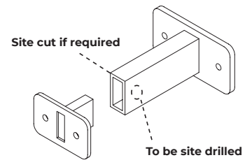
Tee Bracket
